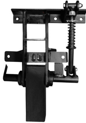
SP 192 PARTIAL MECHANISM FOR KICKER MULTIPLAYER
